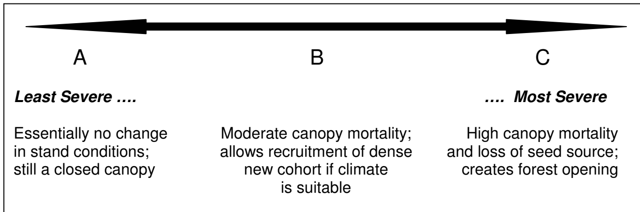
Figure 2. Continuum of potential fire severity and fire effects on forest structure in a small patch (an acre or so) of ponderosa pine forest having a relatively closed canopy before the fire.
